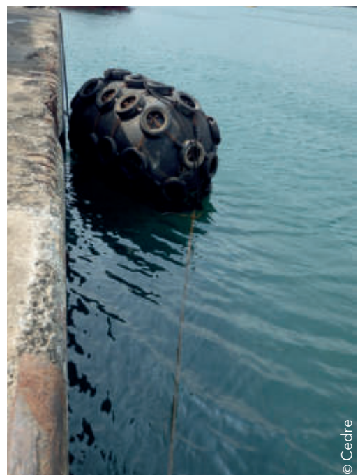
Yokohama fenders used to allow approach between two ships
