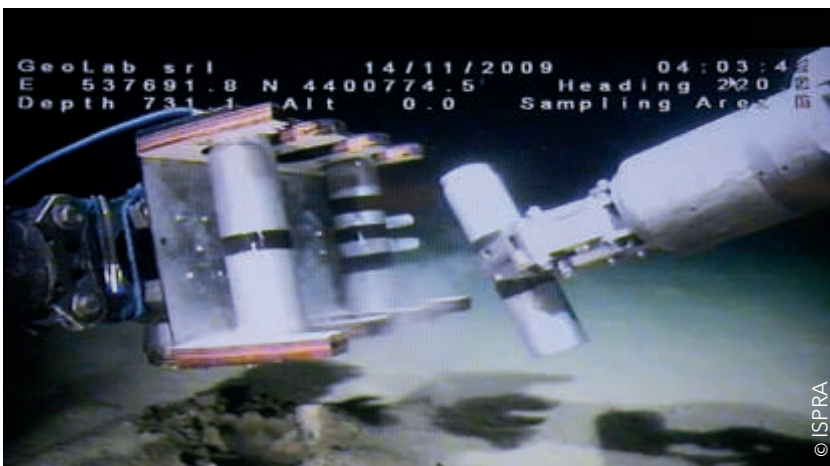
Sediment sampling with a ROV on the deep seafloor
